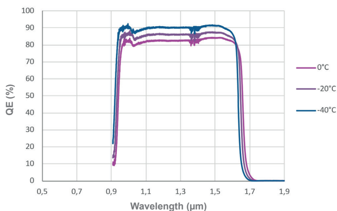
QUANTUM EFFICIENCY
