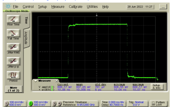
10,000ps Pulsewidth @ Clock Freq. 1MHz
