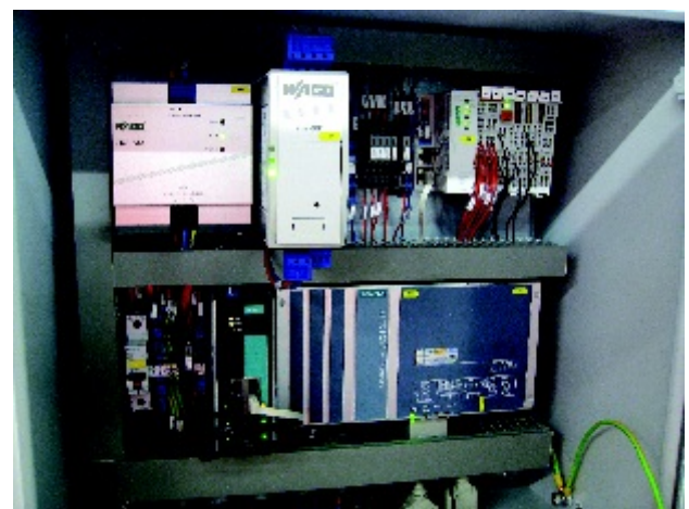
Electronics Cabinet with Embedded Computer and Peripheral Components
