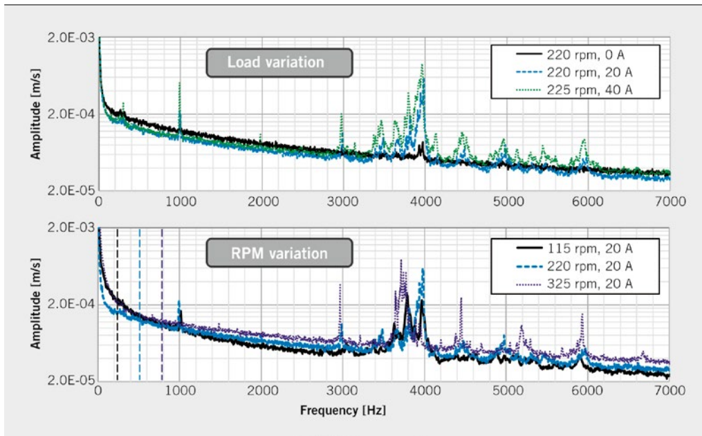
FIGURE 4 Vibration amplitude spectra of different operating points averaged over the measurement surface (© OVGU)
