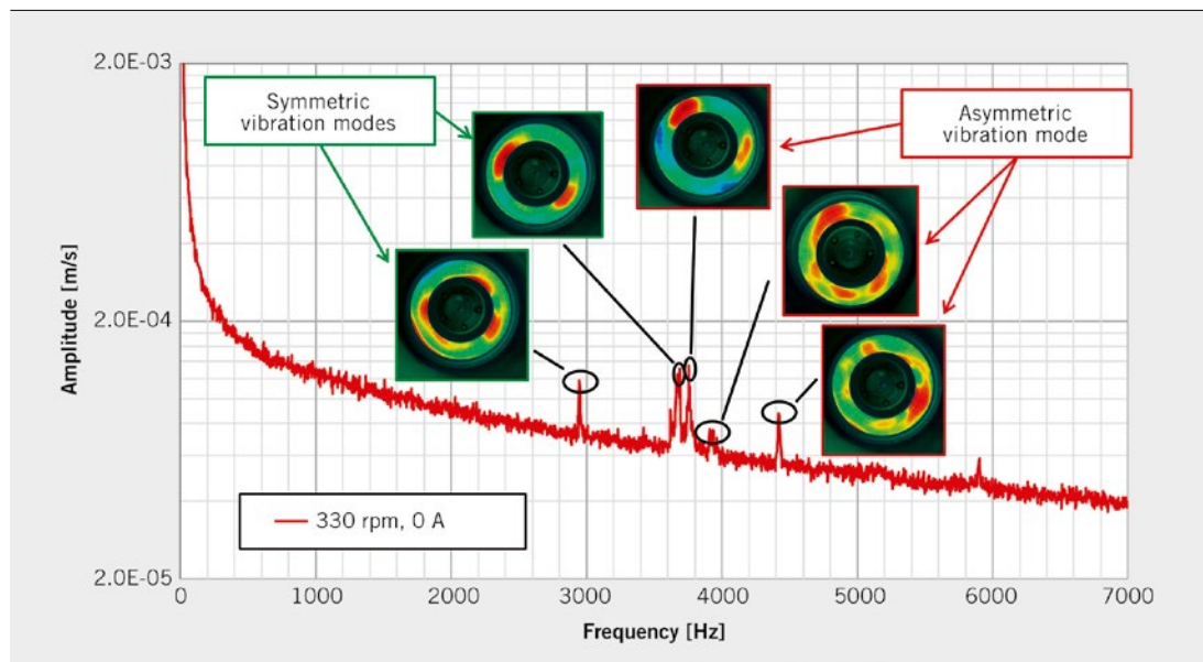
FIGURE 5 Spectrum of the vibration amplitudes averaged over the measurement grid with conspicuous vibration modes during idling (© OVGU)
