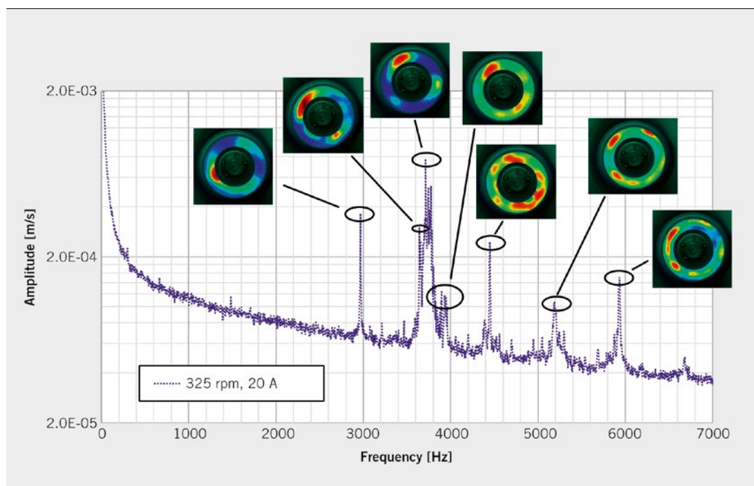
FIGURE 6 Spectrum of the vibration amplitudes averaged over the measurement grid with conspicuous vibration modes at a stationary operating point (© OVGU)
