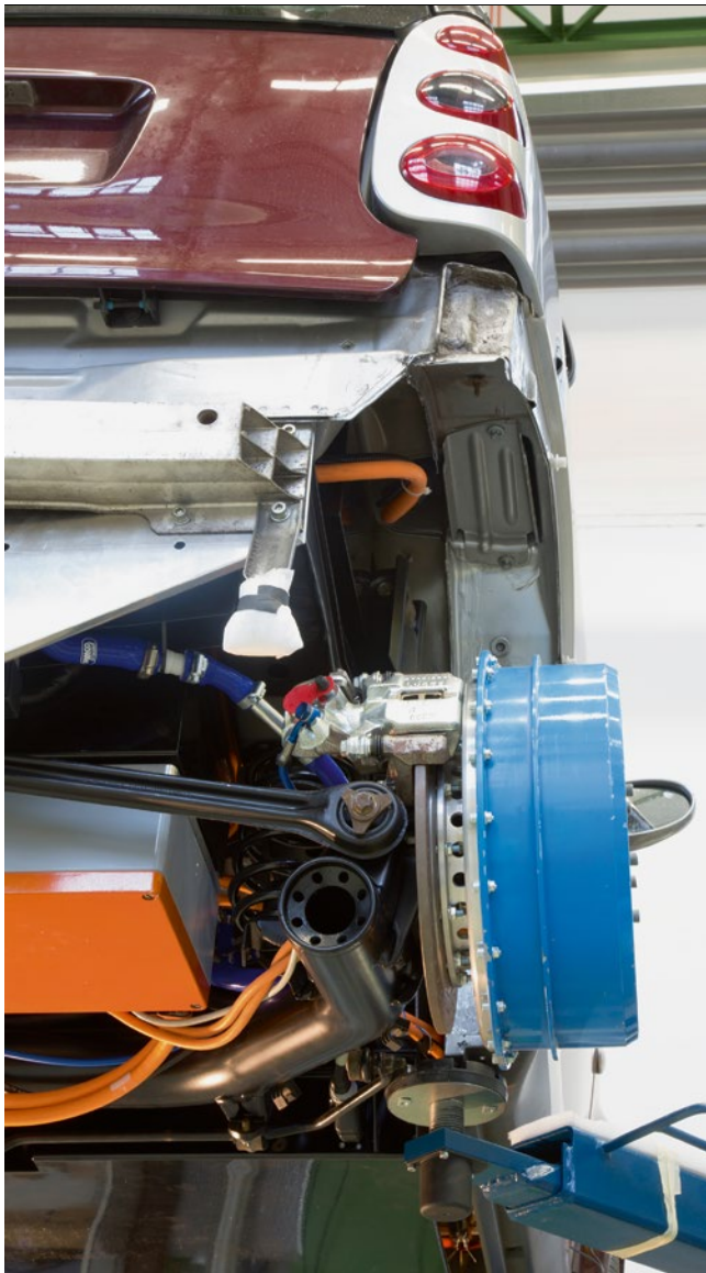
FIGURE 1 Wheel hub motor implemented in the research vehicle Editha 3 (© OVGU)
