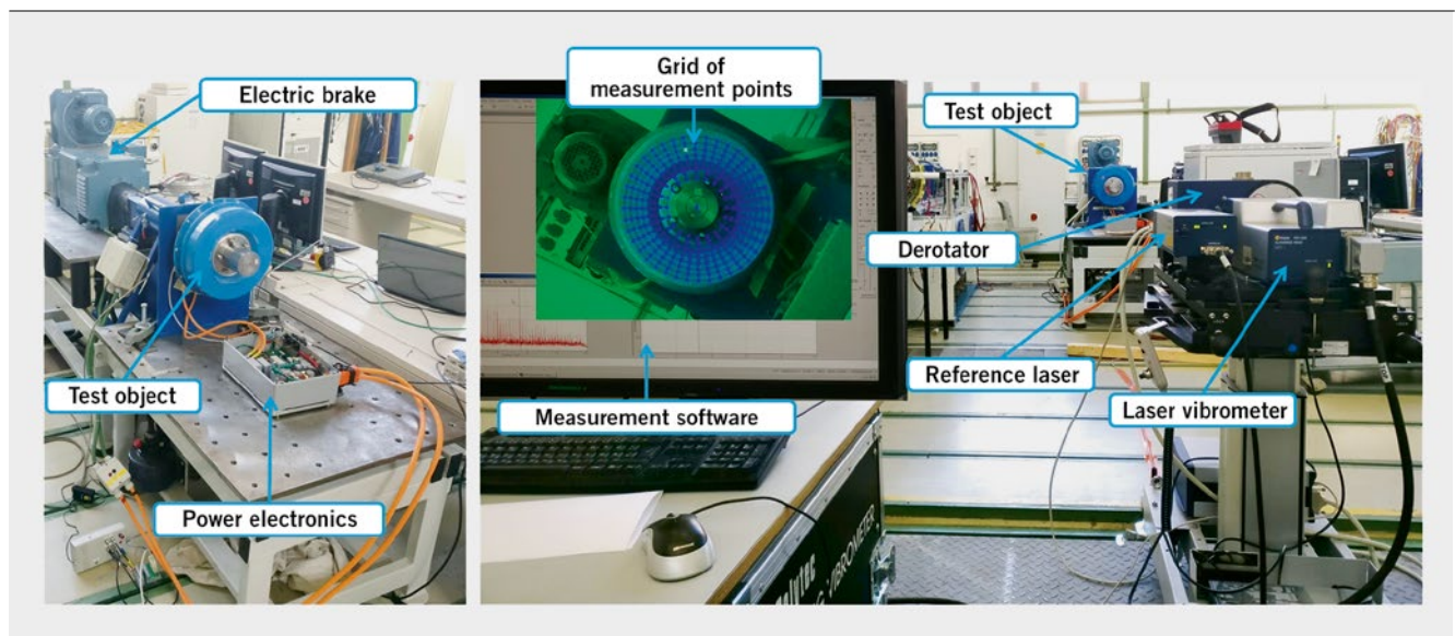
FIGURE 3 Experimental setup for the vibration analysis of the running wheel hub motor (© OVGU)
