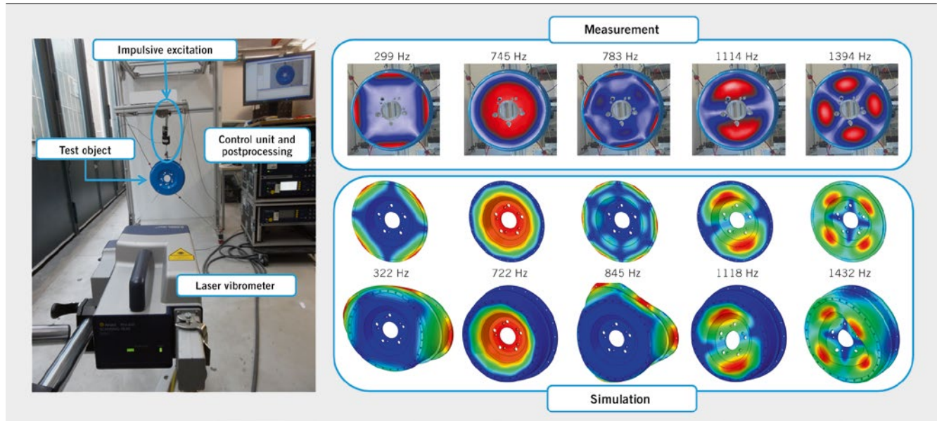
FIGURE 2 Experimental setup used for validation measurement (left) and results of experimental and numerical vibration analysis (right) (© OVGU)
