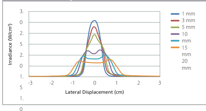
Irradiance vs. Working Distance for AC2 Series – 395 nm
