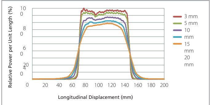
AC2 Series Uniformity – 395 nm
